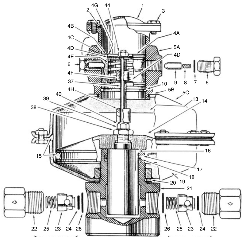
OUTLET Check Valve Assembly 10:1 through 100:1
